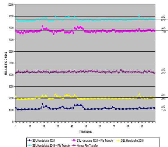
Figure 1. File transfer timing measurements with and without SSL protection.
